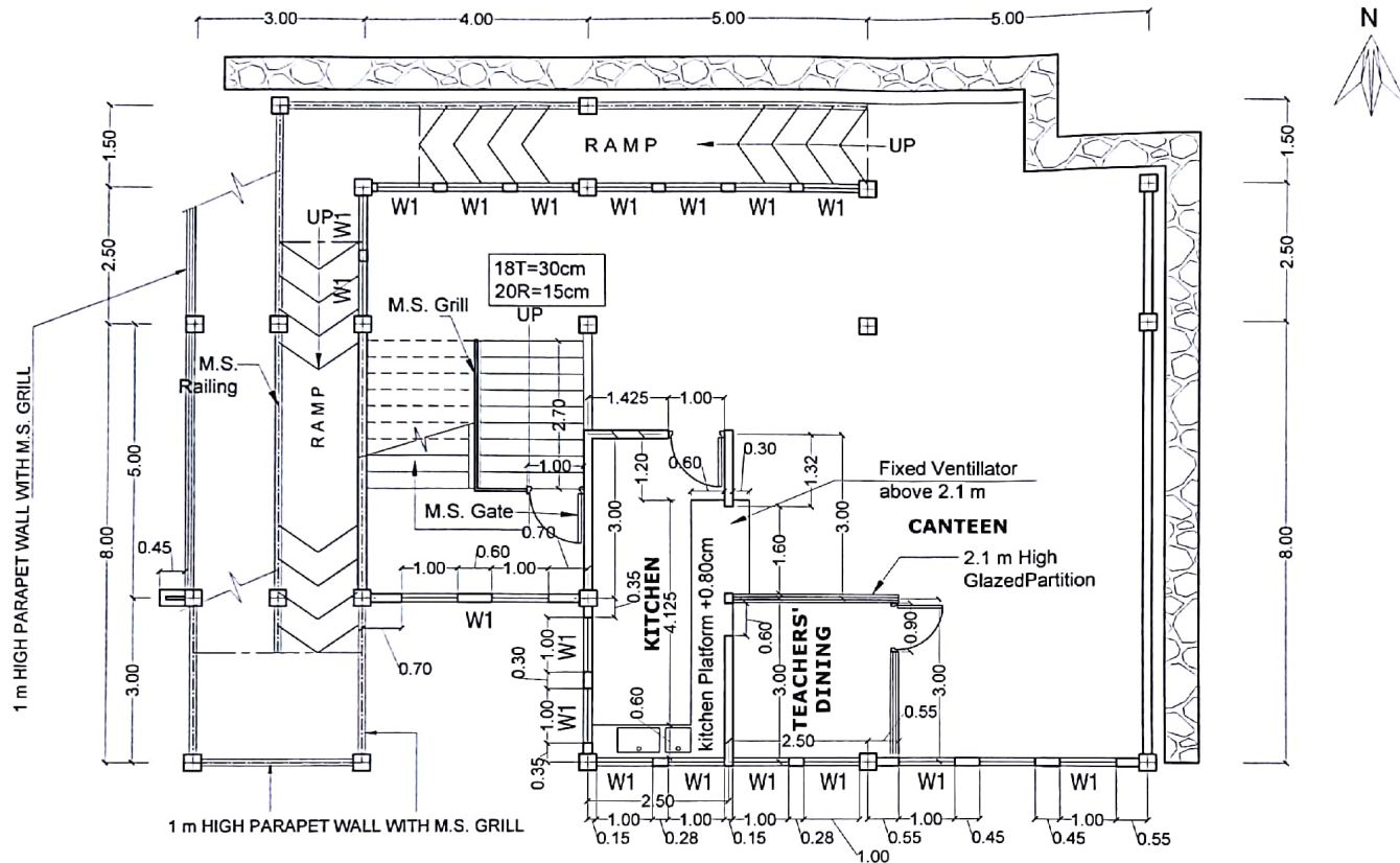
GROUND FLOOR PLAN AT LEVEL+86m
